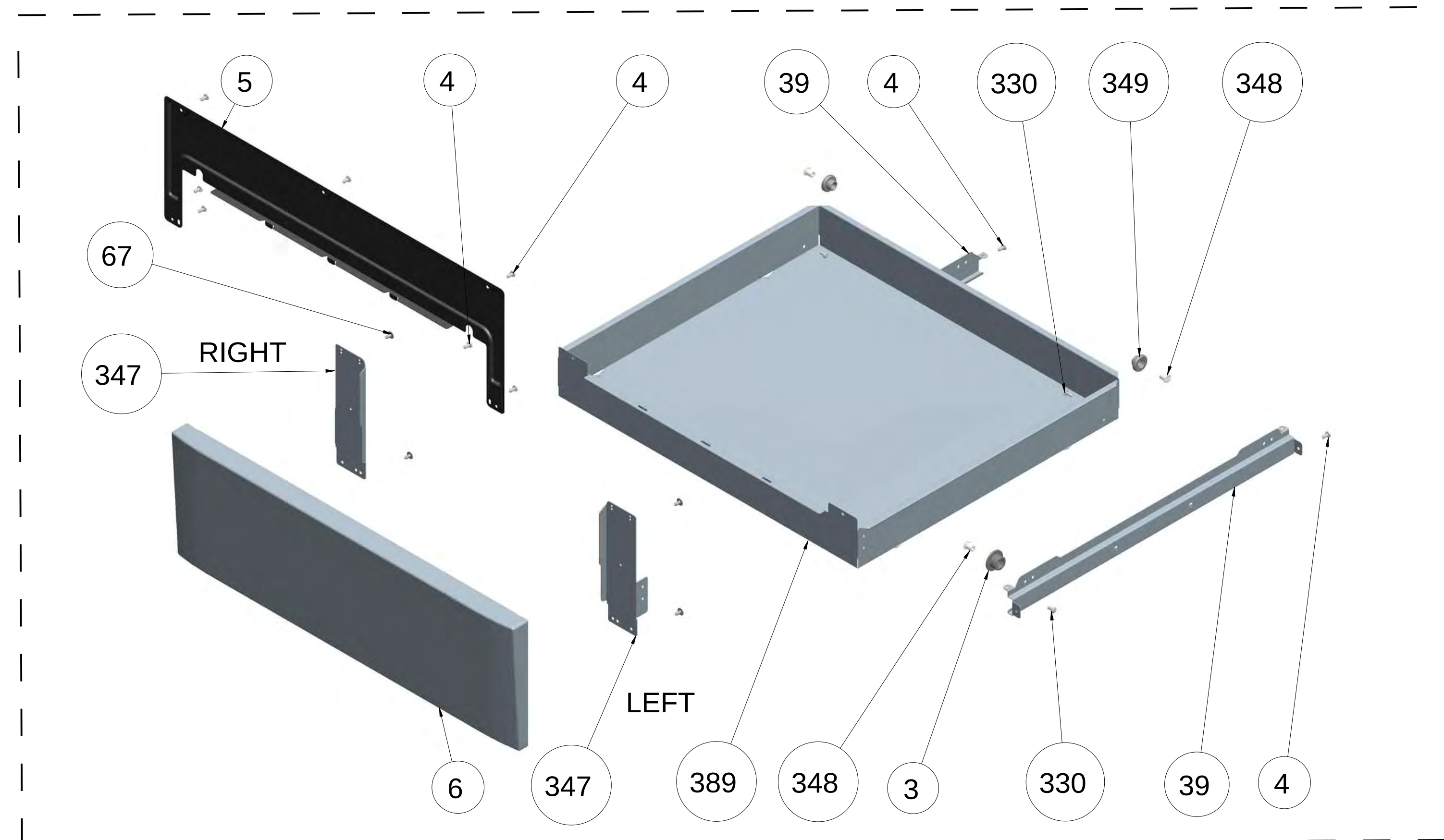
4WG DRAWER ASSEMBLY (OPTIONAL)
