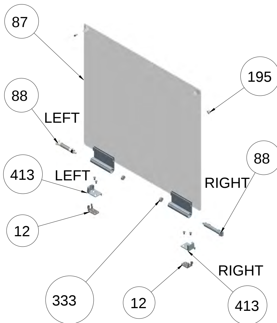
GLASS LID WITH BUMPER OPTIONAL
